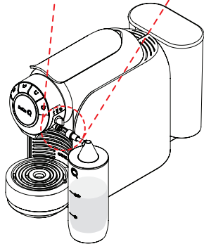
Fig. 20: Connect the milk tank to the milk system.
